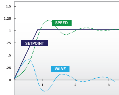
Typical PID Response CURRENT
